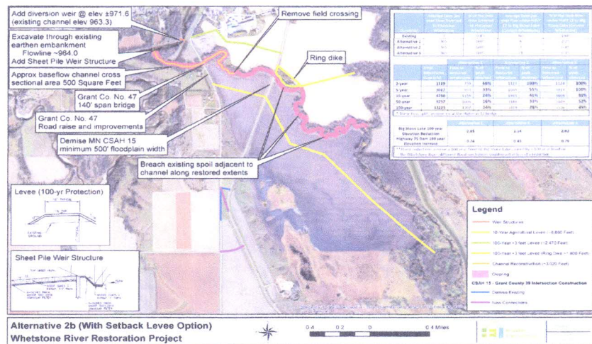
Figure 1: Alternative 2b (With Setback Levee Option)
